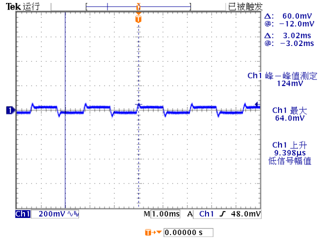
Figure 5, 50% - 75% load dynamic
