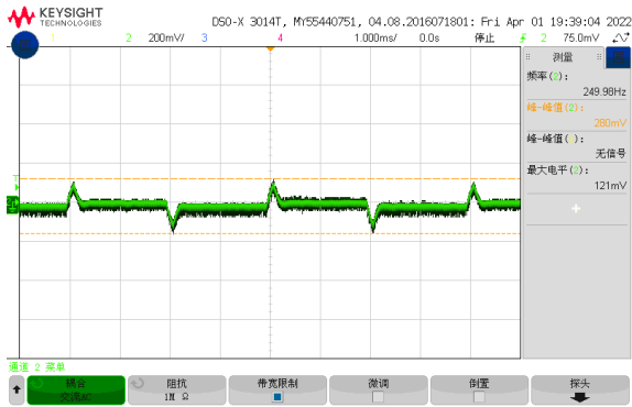
Figure 4, 25% - 50% load dynamic
